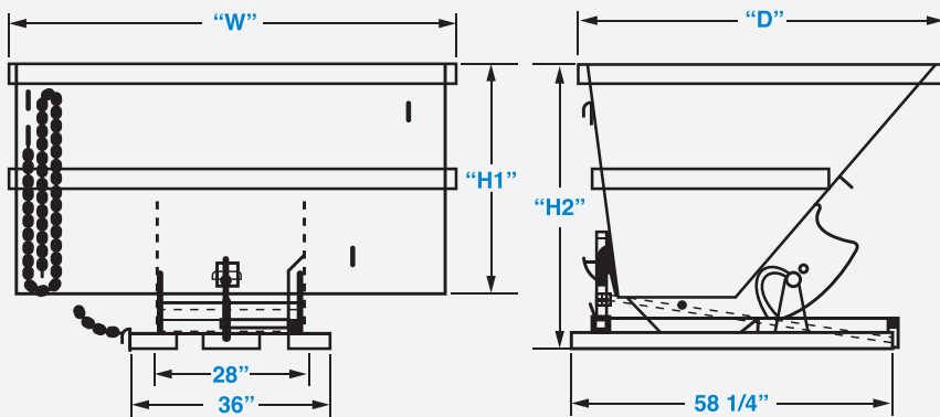
BUMPER RELEASE STYLE FRONT & SIDE VIEWS
