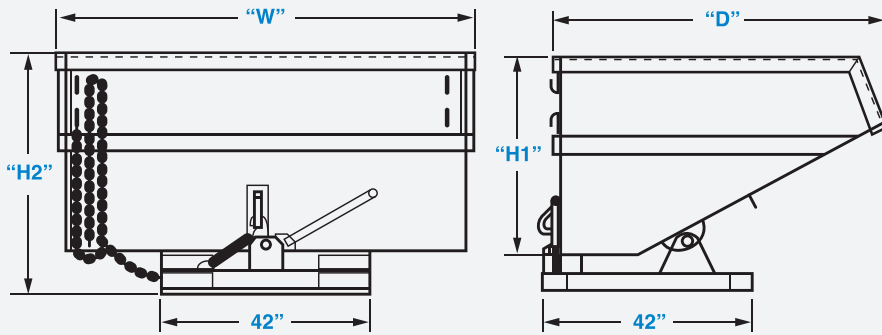
PIVOT STYLE FRONT & SIDE VIEWS
