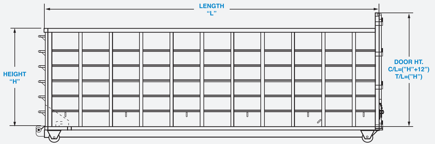
VIEW ABOVE 22 X 6.5 STD 40YD
