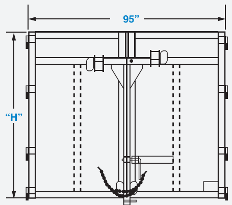
STD. T - LOCK DOORS
