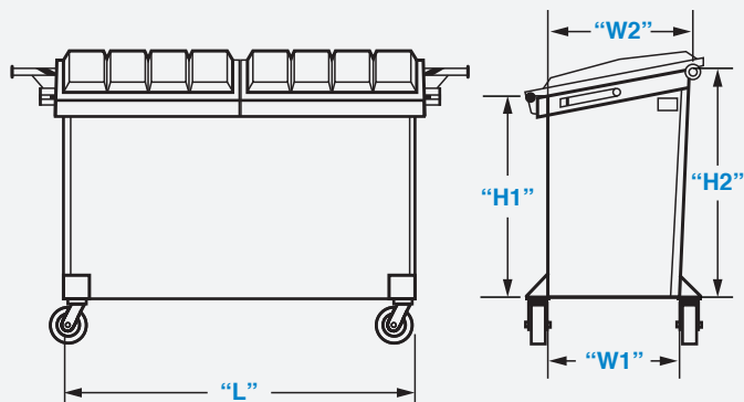
1 YARD REAR LOAD FRONT & SIDE VIEWS
