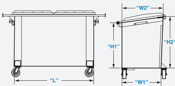
1.5 YARD REAR LOAD FRONT & SIDE VIEWS
