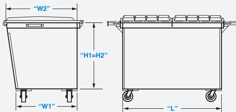
2 YARD REAR LOAD FRONT & SIDE VIEWS
