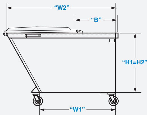
3 YARD REAR LOAD FRONT & SIDE VIEWS
